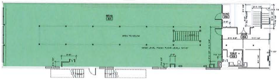
2 SECOND FLOOR PLAN SCALE: 1/8" = 1'-0"
