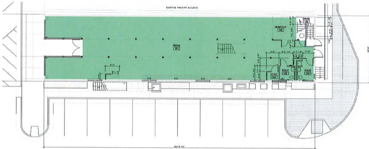
1 FIRST FLOOR PLAN SCALE: 1/8" = 1'-0"
