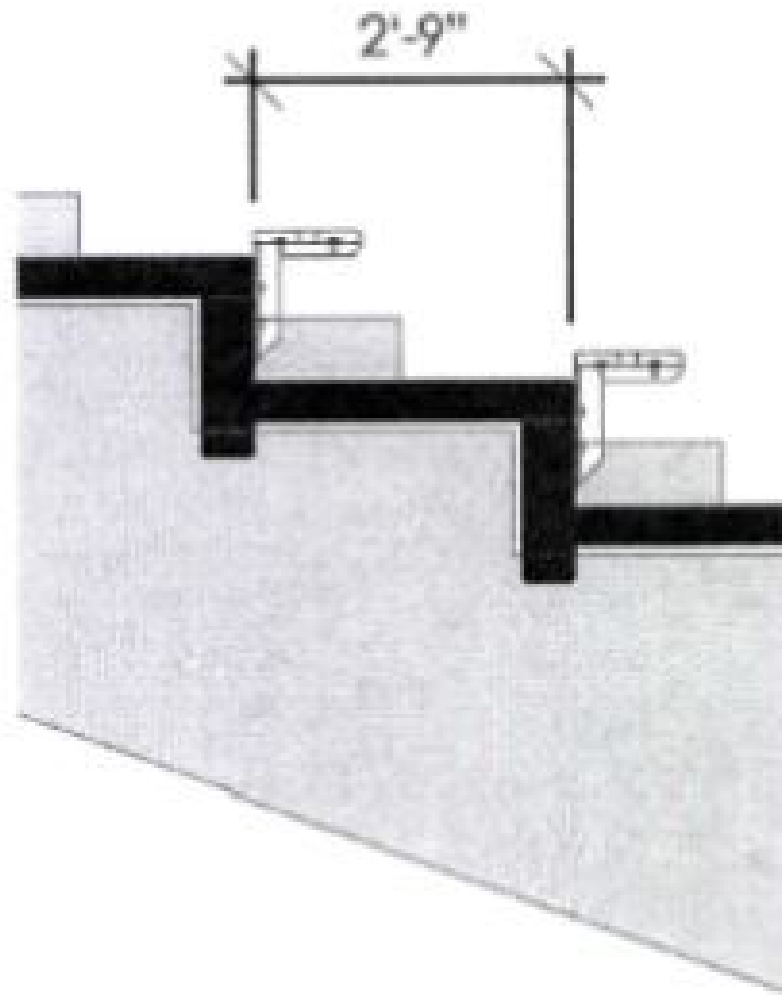
Typical Lower Deck Section Diagram
