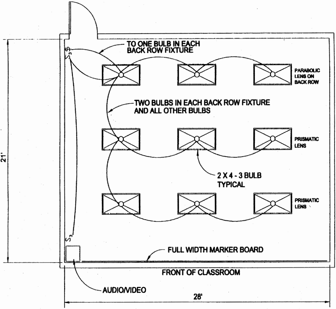
Figure 34 Classroom Lighting Detail
