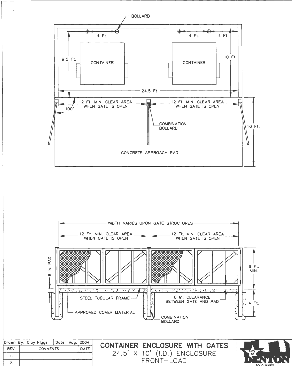
Figure 11 Outdoor Solid Waste Enclosure with Gates Detail
