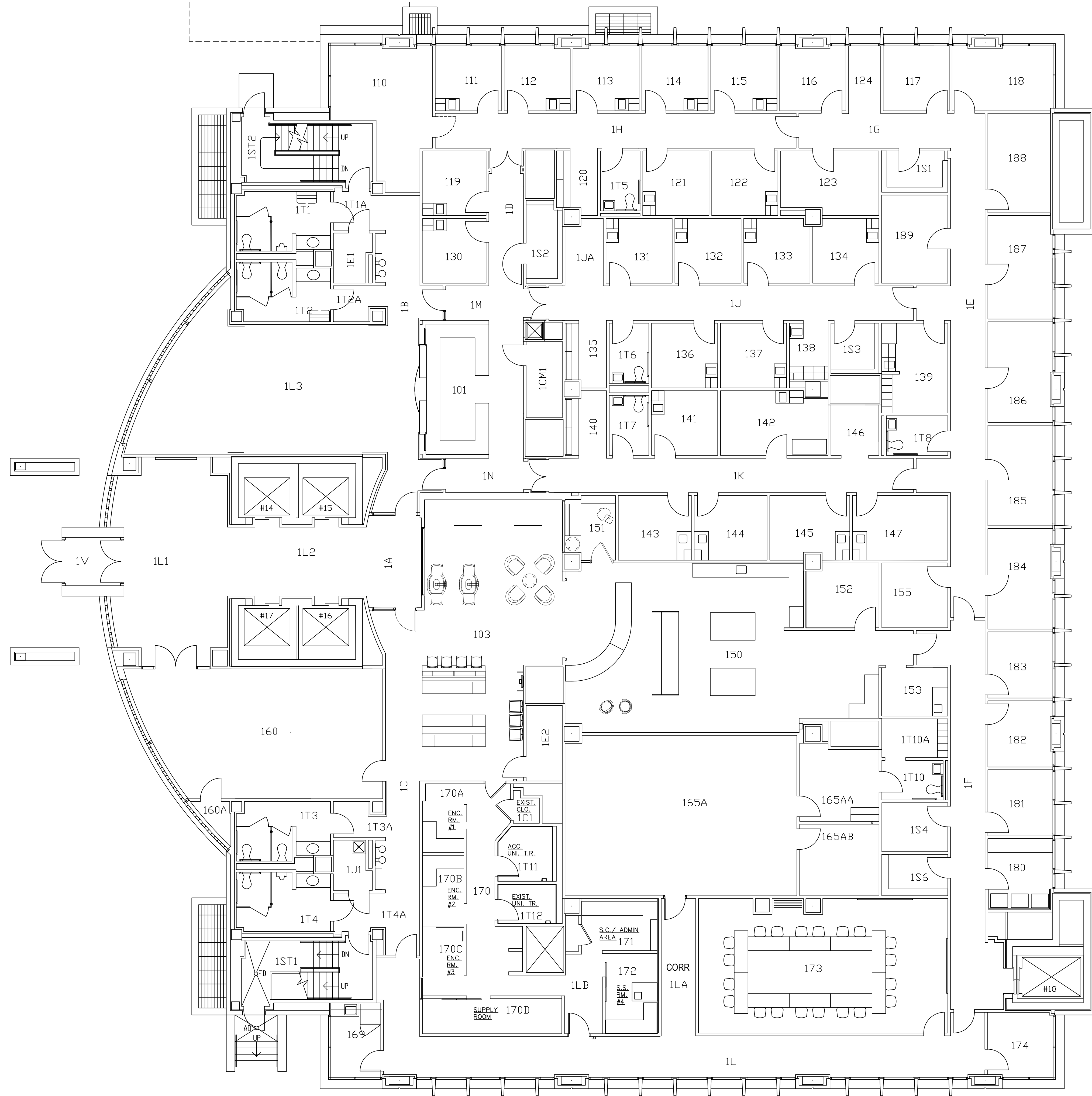
1 HEALTHCARE PAVILION, LEVEL 1 FLOOR PLAN
